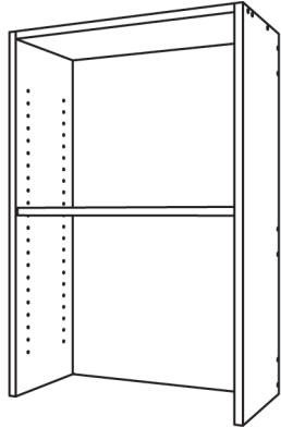
CM440 Open Hutch Cabinet • Specify number of adjustable shelves • Interior surface shall be as listed on order form unless noted differently
