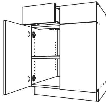
CM222 Two-Door Base Cabinet - Two-Drawer • Specify type and number of shelves per opening on order form
