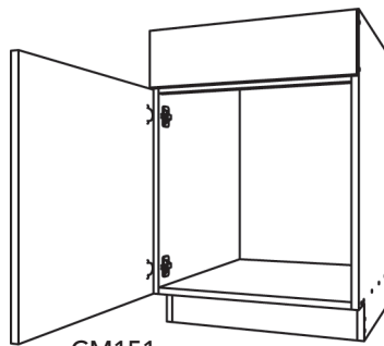
CM151 One-Door Base Cabinet - False Front • Specify false front height • Apron behind FF and hangs 1/2" lower
