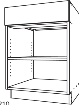
CM210 One-Drawer Open Base Cabinet • Specify opening height • Interior surface shall be as listed on order form unless noted differently
