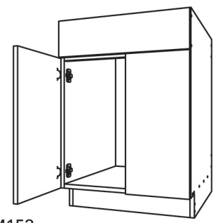
CM152 Two-Door Base Cabinet - False Front • Specify false front height • Apron behind FF and hangs 1/2" lower
