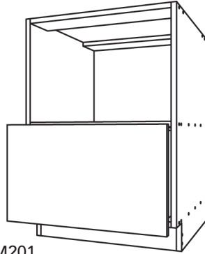
CM201 One-Drawer Open Base Cabinet • Specify opening height • Interior surface shall be as listed on order form unless noted differently
